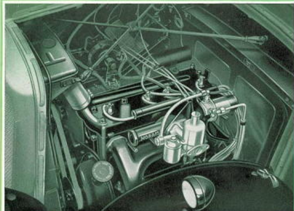
All components of the 12 h.p. engine of the Morris 10-cwt. Light Van are readily accessible, the distributor included. The accessible engine oil filler will also be observed
